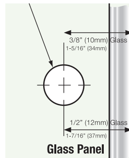
45° Mitered Panel
