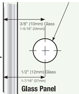
45° Mitered Panel
